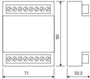
DALI-CV-HP (L406MA0GT4A04) DALI-CC-HP (L405MA0GC4A04)
